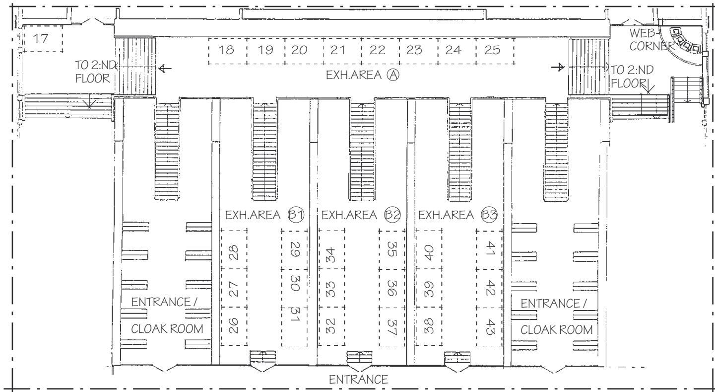
FLOOR 1
